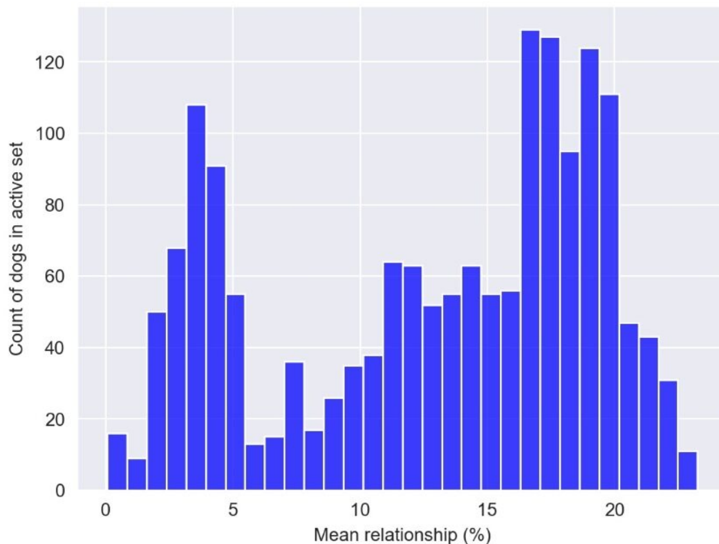
Figure 9 Histogram of the average relationships between dogs in the current breeding population (bitches born in last 8 years and dogs born in last 10 years, total of 1,703 dogs)
