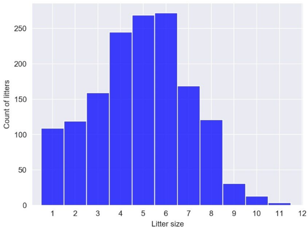
Figure 5 Distribution of litter size
