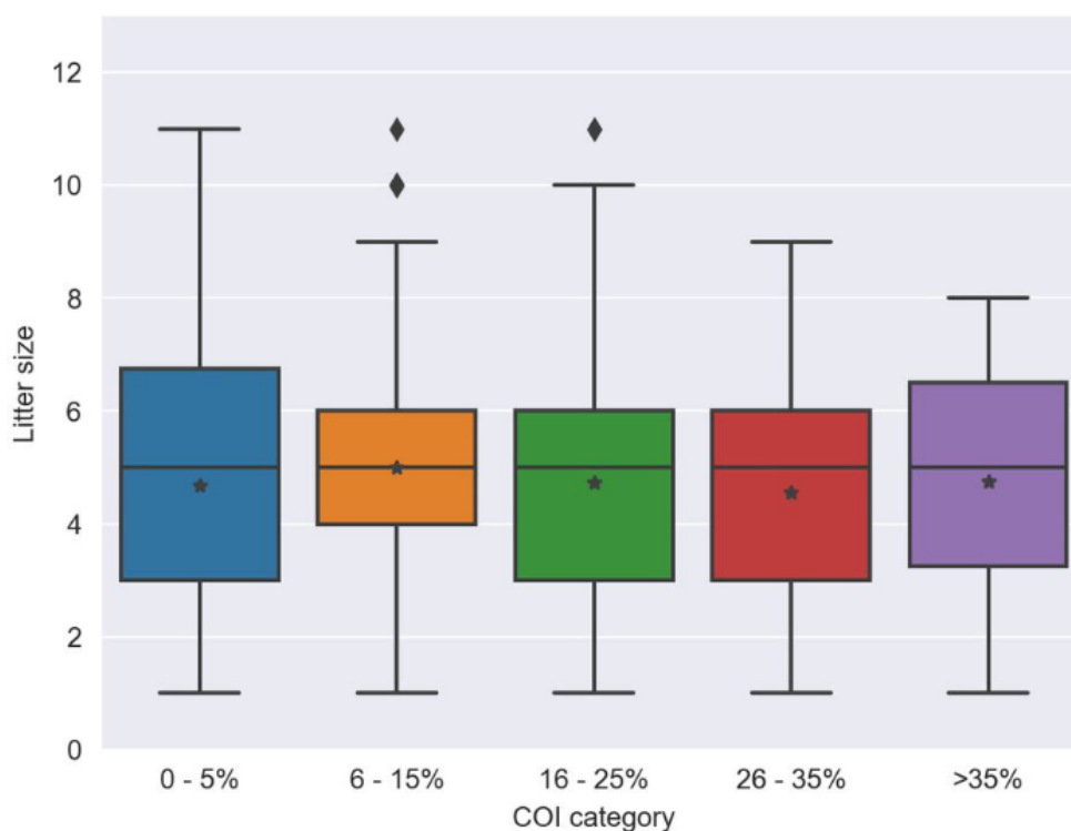
Figure 7 Boxplot of litter size distribution by category of COI. The number of litters in the particular categories were: 0-5% = 216, 6-15% = 805, 16-25% = 412, 26-35% = 74, >35% = 4
