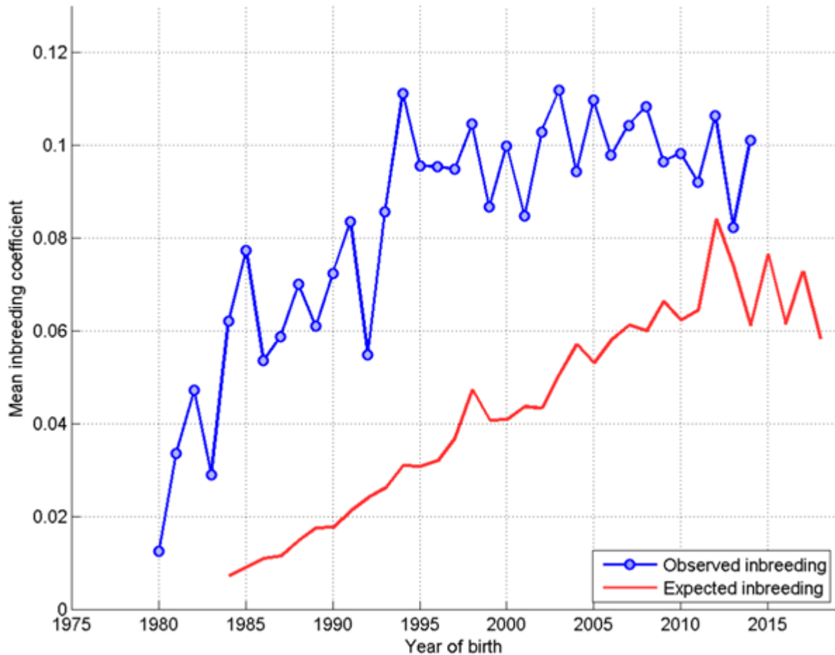
Figure 41: Annual mean observed and expected inbreeding coefficients.
