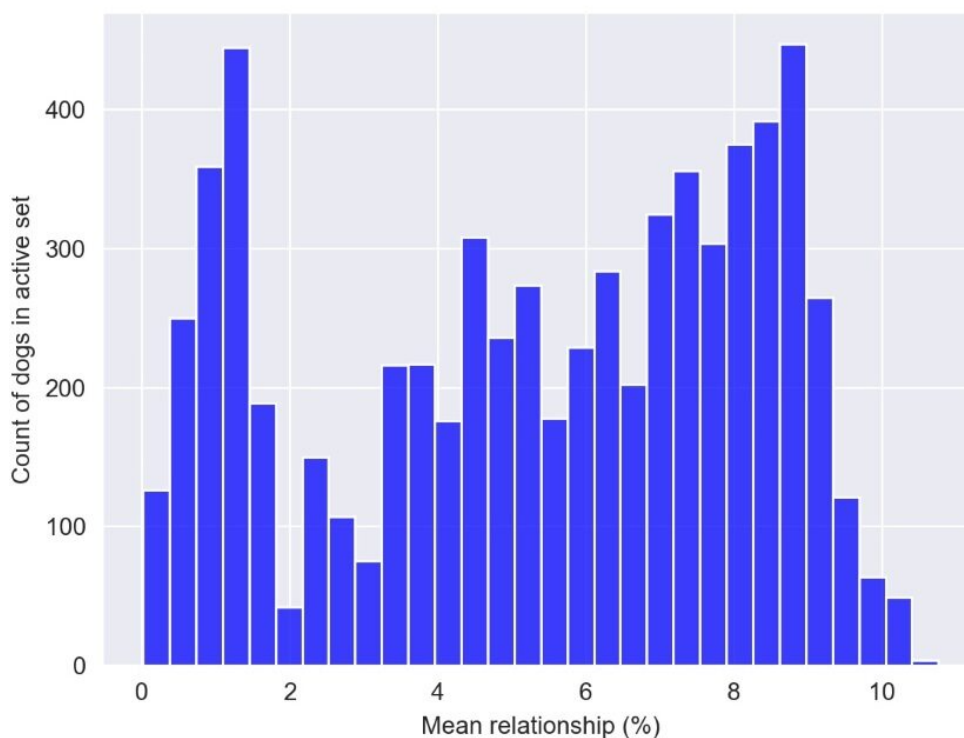
Figure 9 Histogram of the average relationships between dogs in the current breeding population (bitches born in last 8 years and dogs born in last 10 years, total of 6,765 dogs)
