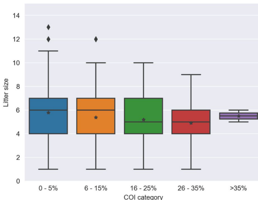
Figure 7 Boxplot of litter size distribution by category of COI. The number of litters in the particular categories were: 0-5% = 1,133, 6-15% = 1,028, 16-25% = 300, 26-35% = 49, >35% = 2
