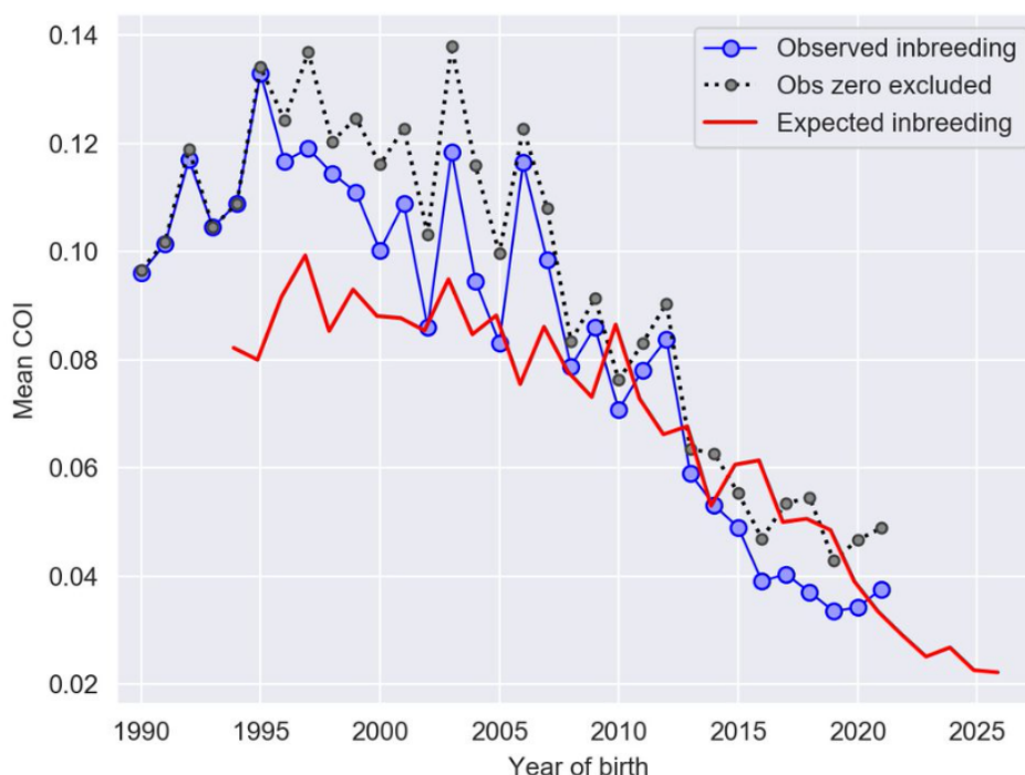
Figure 6 Annual mean observed and expected inbreeding coefficients
